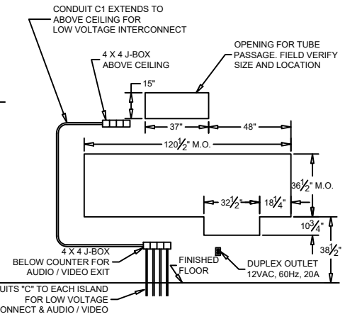
MASONRY DETAIL (FOR MODEL 310D U.L. WINDOW)
